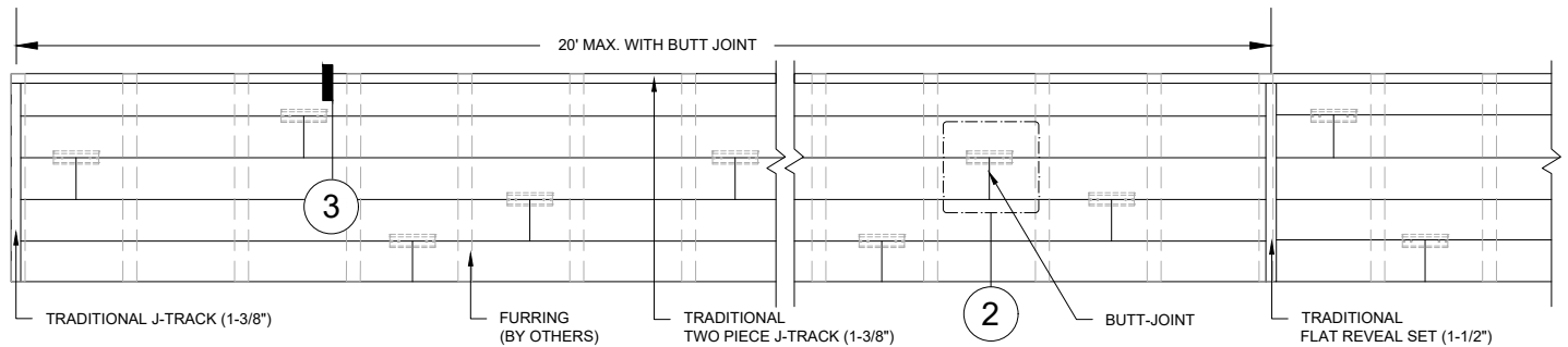
1 ELEVATION WITH MULTIPLE BUTT-JOINTS SCALE 1:30
