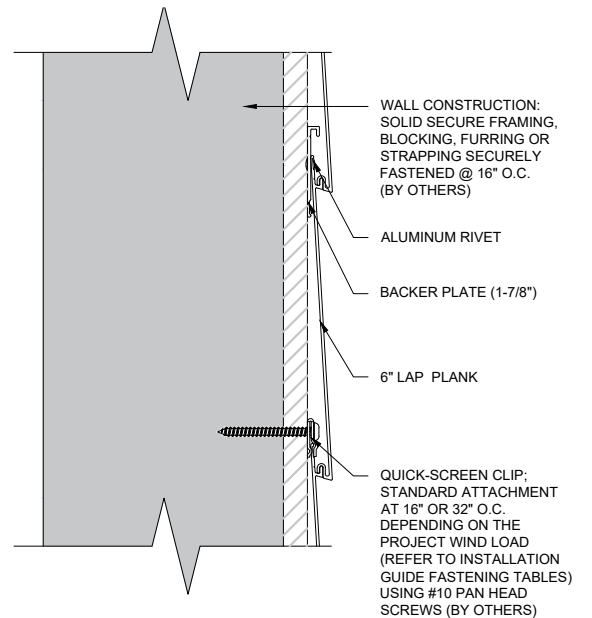
3 SECTION SCALE 1:4
