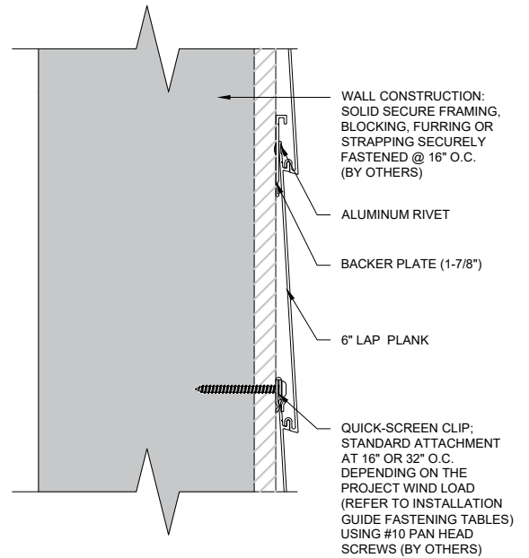
3 SECTION SCALE 1:4
