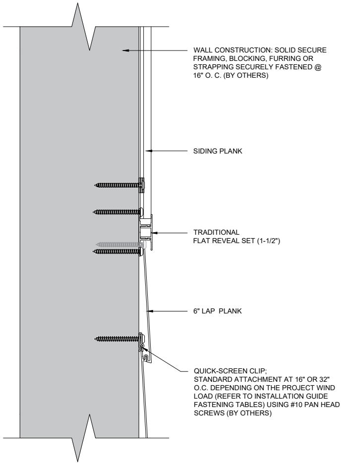
SECTION VIEW
