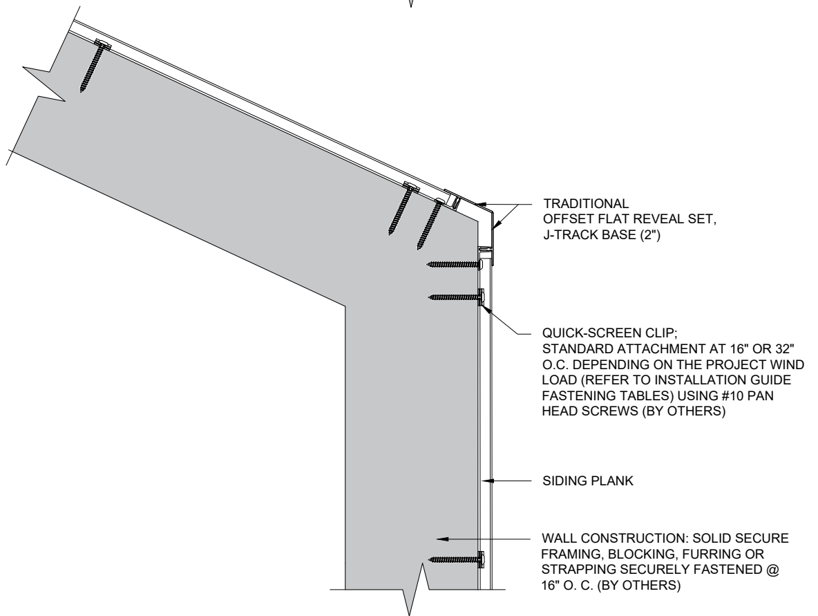
PLAN VIEW
