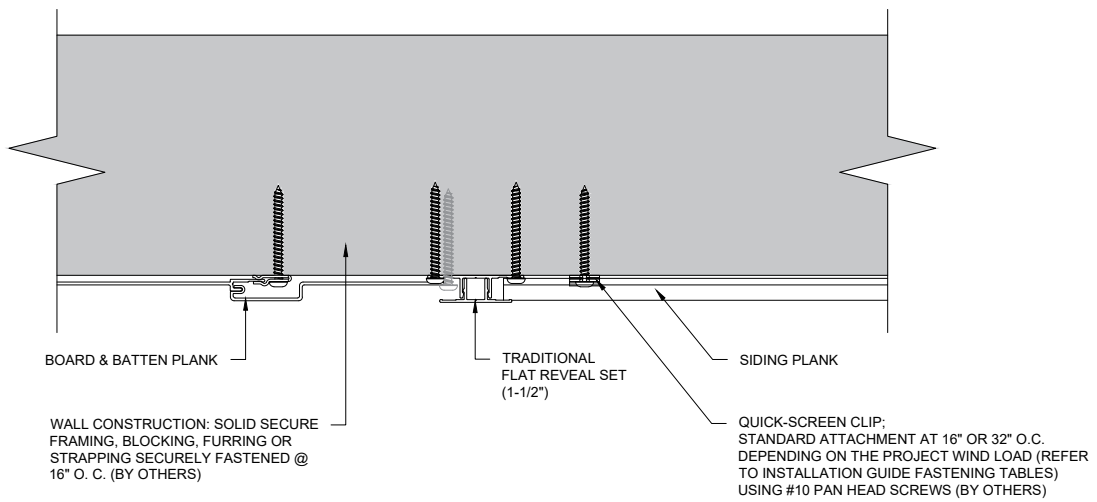
PLAN VIEW
