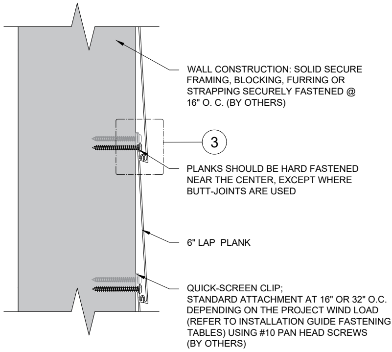
2 SECTION SCALE 1:4
