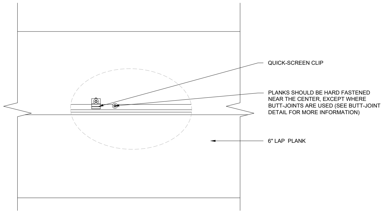
1 ELEVATION SCALE 1:4
