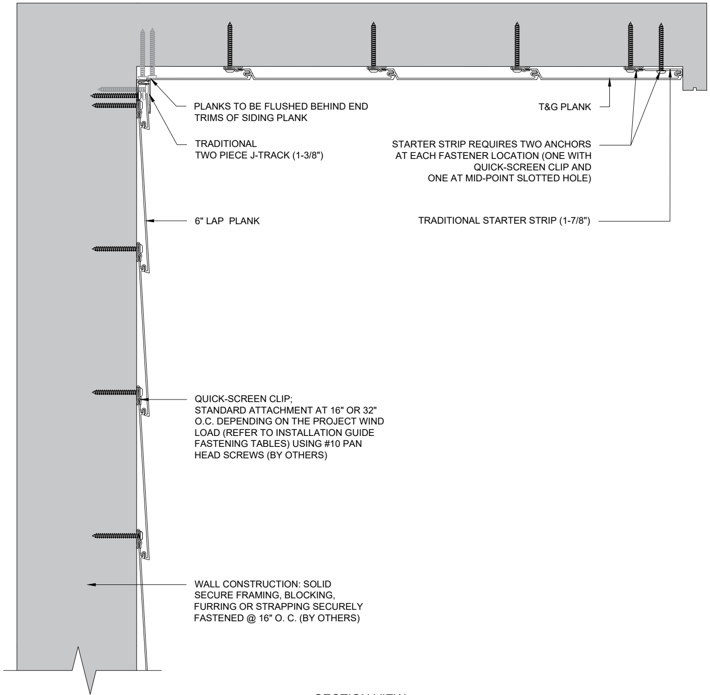
SECTION VIEW
