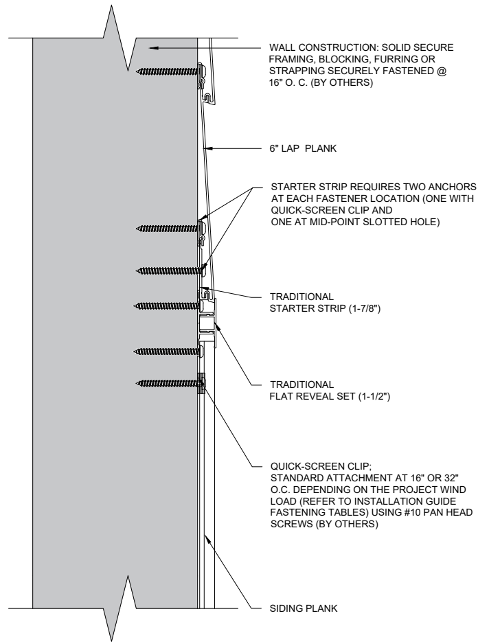
SECTION VIEW
