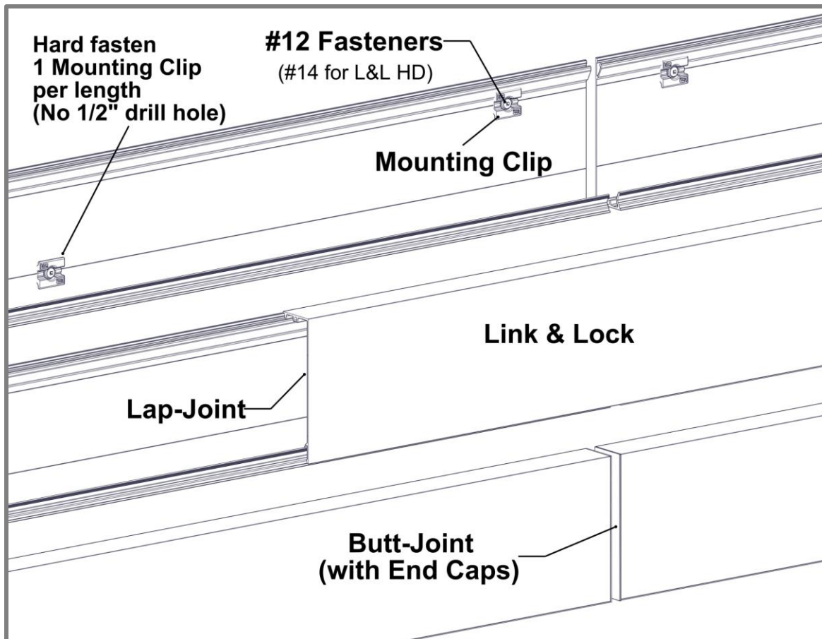
Detail A
