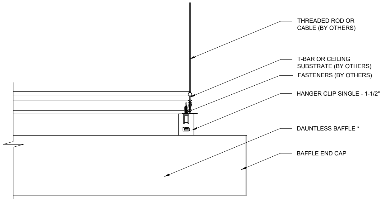
SECTION B-B
