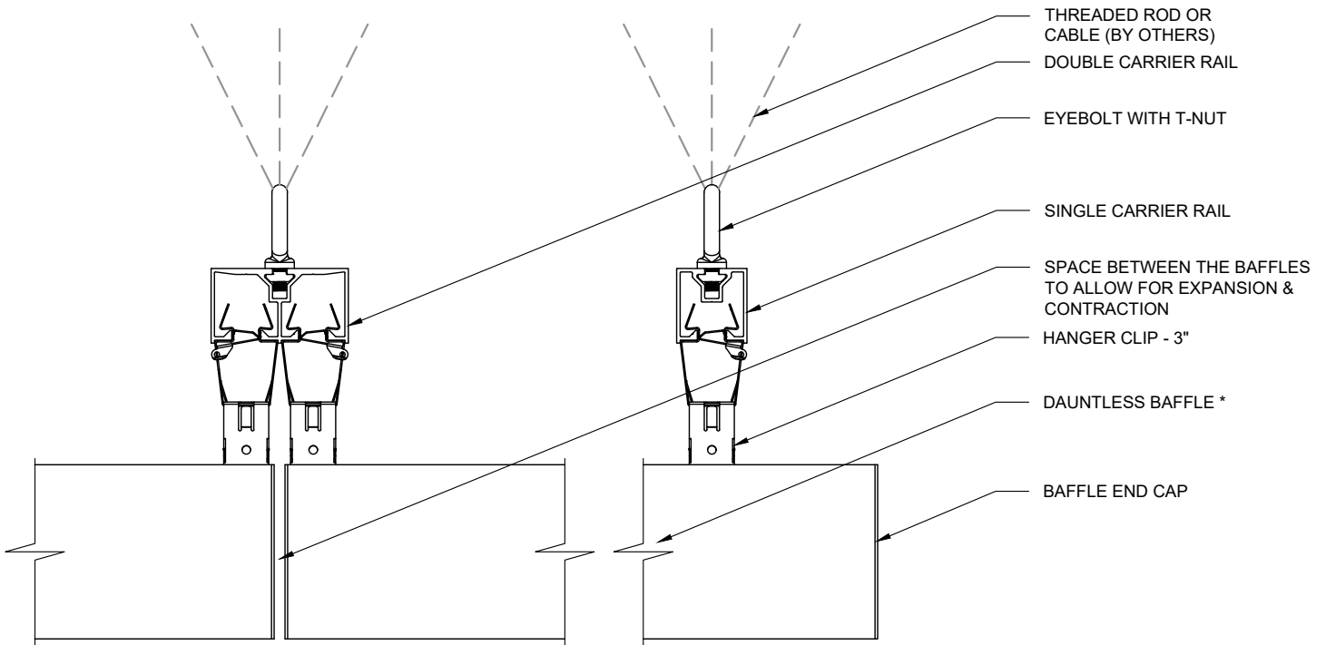
SECTION B-B
