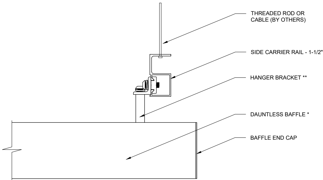
SECTION B-B
